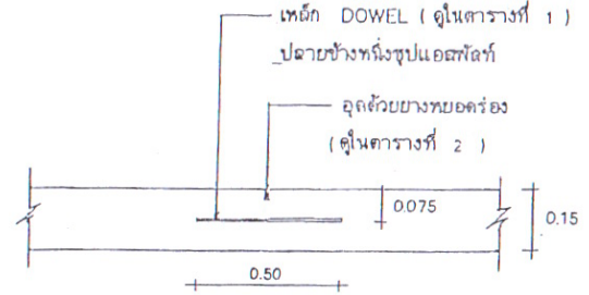
CONTRACTION JOINT
